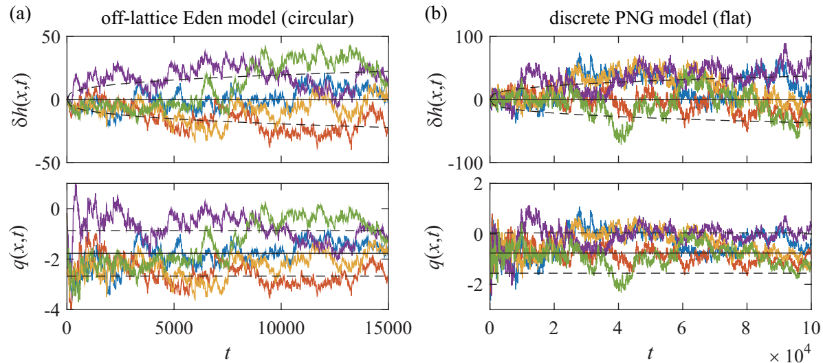
Figure 3. Typical time series of \delta h(x,t) and q(x,t) for the circular (a) and flat (b) cases. Numerical data are shown here, for which much longer time series are available. The solid and dashed black lines indicate the mean value and the range of the standard deviation, respectively, valid for large t . It is given by \pm(\Gamma t)^{1/3}\sqrt{\langle\chi_i^2\rangle_c} for \delta h(x,t) and \langle\chi_i\rangle \pm \sqrt{\langle\chi_i^2\rangle_c} for q(x,t) , with i = 2 for the circular case and i = 1 for the flat case.
