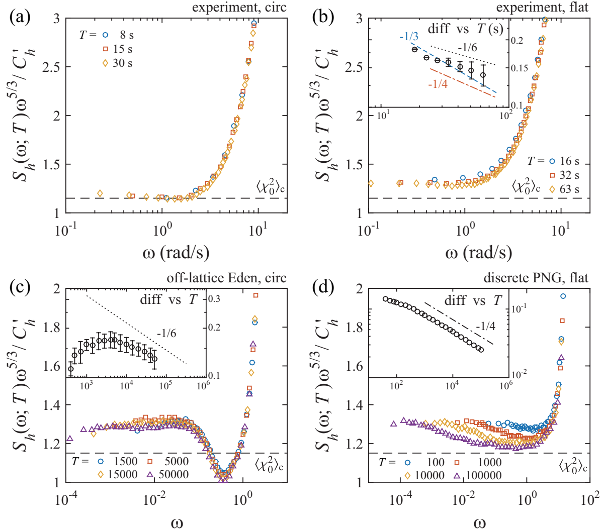
Figure 7. Comparison of the coefficient of the 1/f^\alpha spectrum with the Baik-Rains universal variance, for the liquid-crystal experiments [circular (a), flat (b)], the off-lattice Eden model [circular (c)], and the discrete PNG model [flat (d)]. According to the aging Wiener-Khinchin theorem and the KPZ scaling laws, the ordinate S_h(\omega; T)\omega^{5/3}/C'_h is expected to converge to the Baik-Rains variance \langle \chi_0^2 \rangle_c for T^{-1} \ll \omega \ll \min\{\Delta t^{-1}, \tau_0^{-1}\} , where \Delta t is the time resolution and \tau_0 is a microscopic time scale of the system (see (20)). The dashed lines indicate \langle \chi_0^2 \rangle_c = 1.15039 . In the insets, the difference between S_h(\omega; T)\omega^{5/3}/C'_h and \langle \chi_0^2 \rangle_c is plotted as a function of T . The difference is measured from the value of the plateau region of the main-panel data for (b,c), with errorbars indicating the minimum and maximum in that region; for (d) the difference is measured from the local minimum estimated by cubic fitting. The dotted, dashed-dotted, and dashed lines are guides for the eyes, indicating exponents -1/6 , -1/4 , and -1/3 , respectively.
